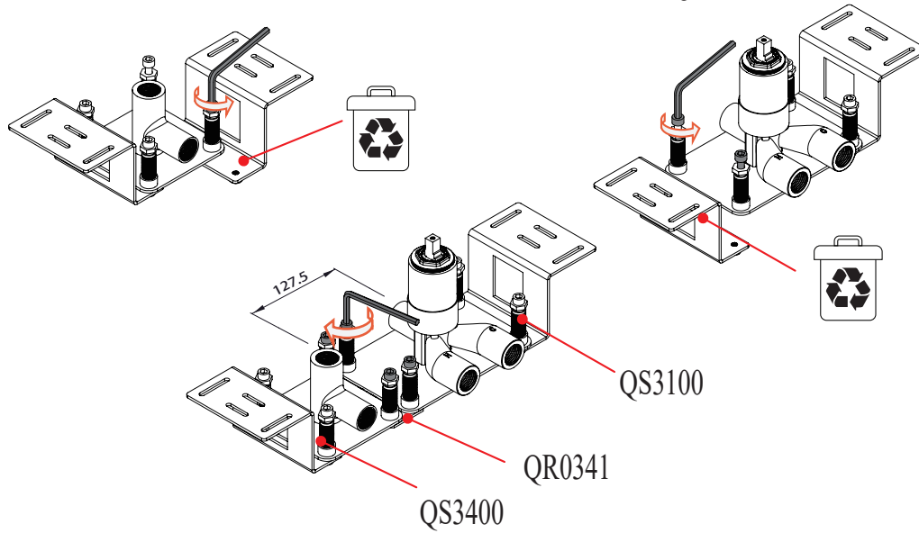
QS3400+QS3100 (Right)
