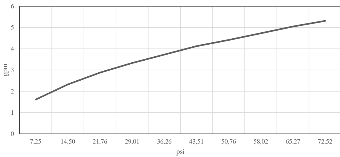
QS3200 flow rate(gpm)
