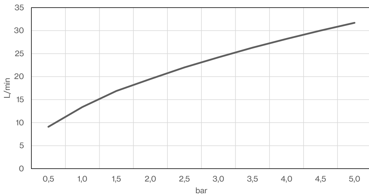
QS5320 flow rate (without aerator)
